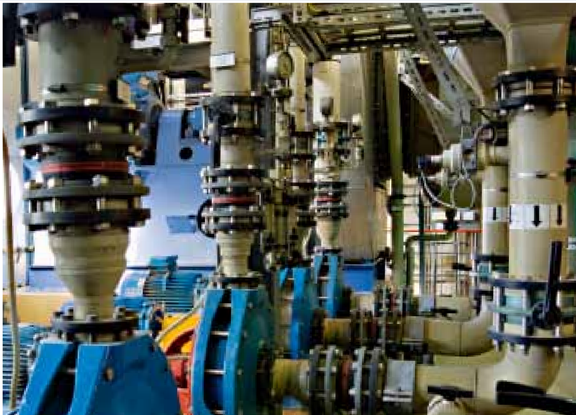
Universal expansion joint, type D110A on the pump suction side DN 250, 10 bar on the pump discharge side DN 150, 10 bar
